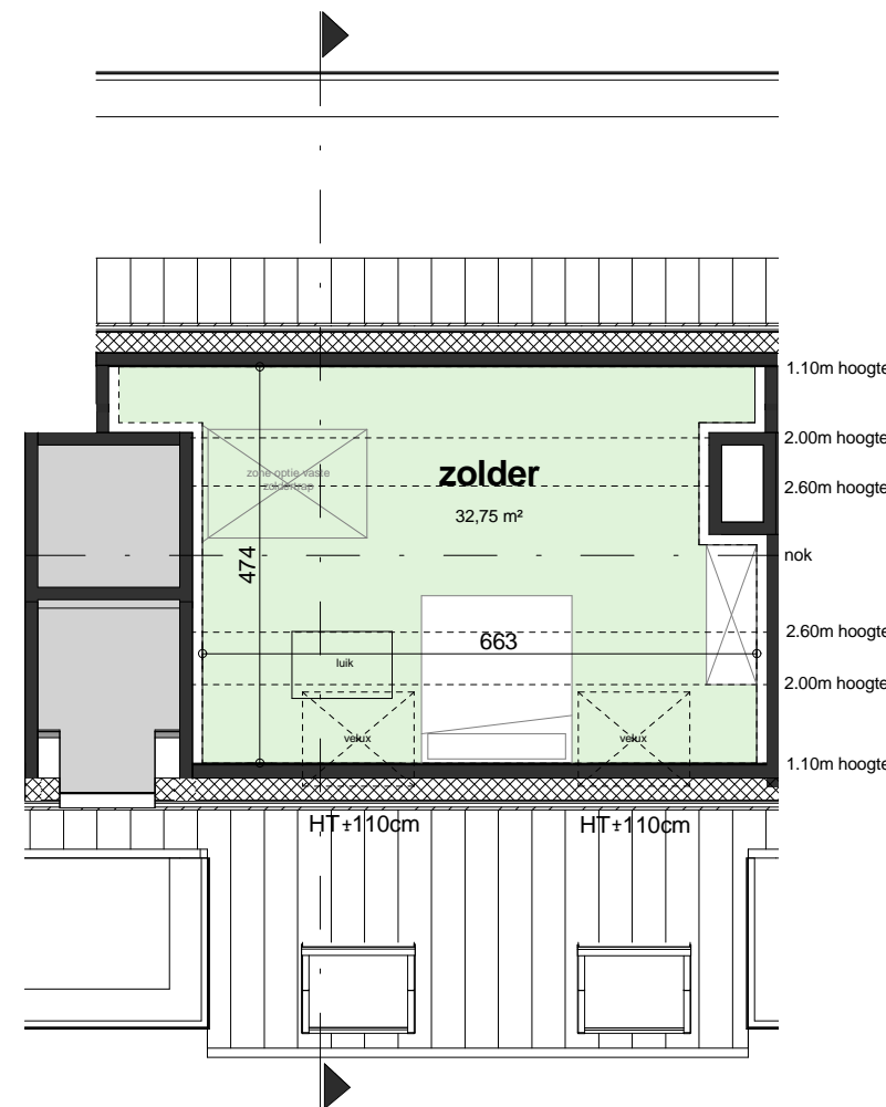
zolder
