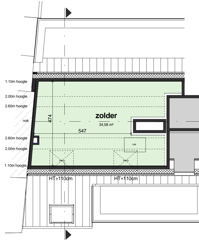
zolder
