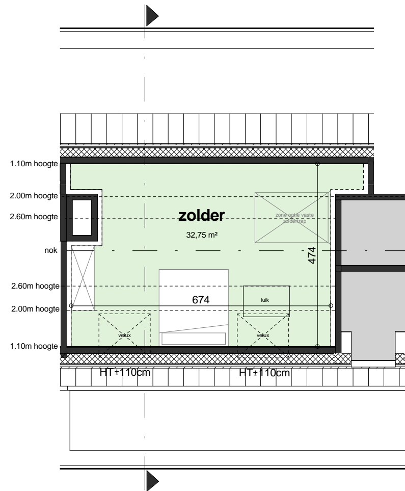
zolder
